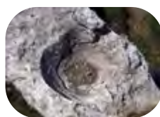
Schists
